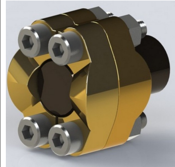
As Per SN 532-1 Flange connection TYPE-D
