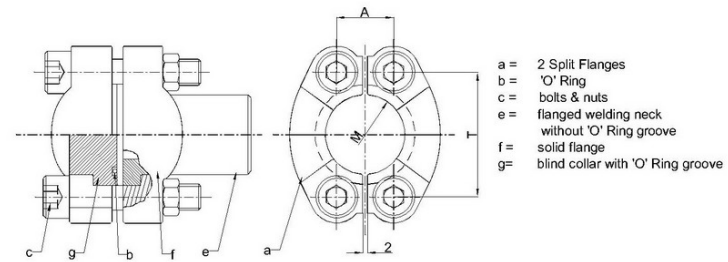
As Per SN 532-1 Flange connection TYPE-D
