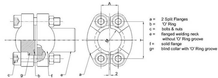
As Per SN 532-1 Flange connection TYPE-D
