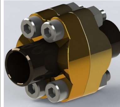
As Per SN 532-1 Flange connection TYPE-B
