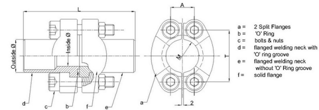
As Per SN 532-1 Flange connection TYPE-B
