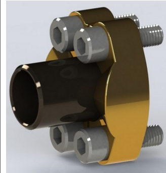
As Per: SN 532-1 Flange connection TYPE-A
