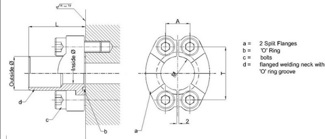
As Per: SN 532-1 Flange connection TYPE-A
