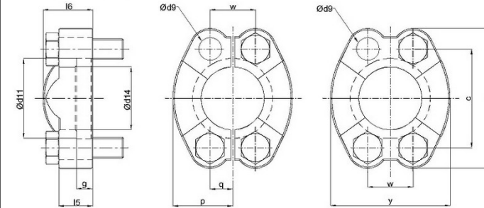
MOUNTING INTERFACE CONFIRMS TO ISO 6162
