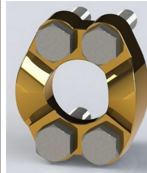
MOUNTING INTERFACE CONFIRMS TO ISO 6162
