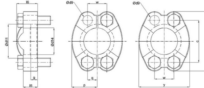
MOUNTING INTERFACE CONFIRMS TO ISO 6162
