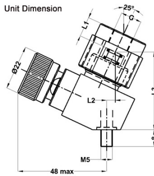
Unit Dimension
