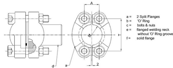
As Per SN 532-1 Flange connection TYPE-C
