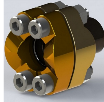
As Per SN 532-1 Flange connection TYPE-C
